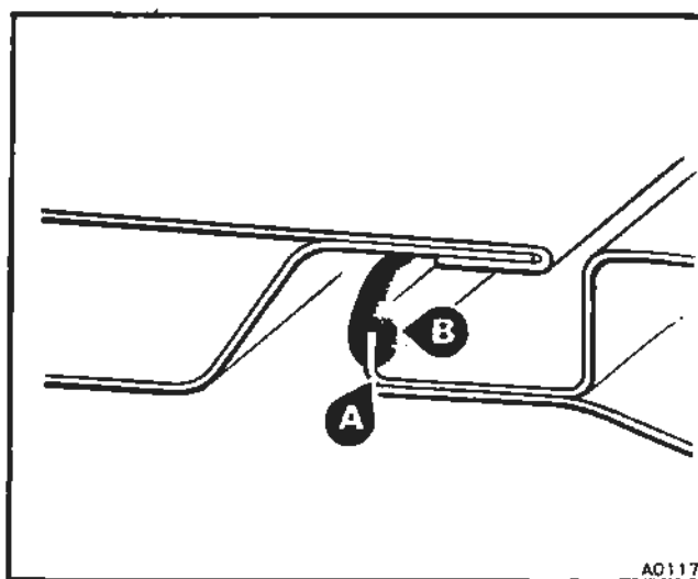
Fig. 2 - Late Cars A Straight edge lip B Late type seal
